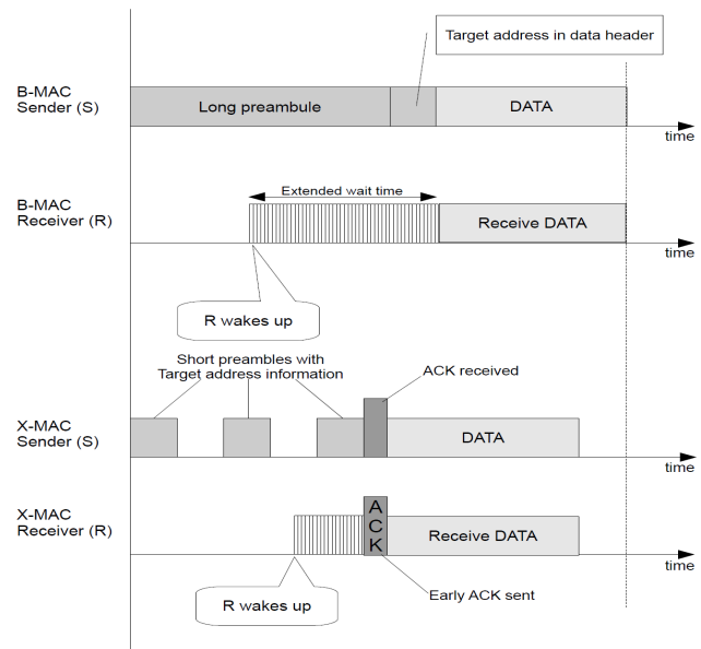
Fig. 1 Comparison of the communication architectures between B-MAC and X-MAC protocols.
